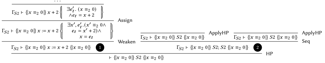
Fig. 2. Simplified proof tree that proves the sub-goal \{x \equiv_2 0\} S_2 \{x \equiv_2 0\} in unrealizability logic. \Gamma_{S_2} denotes the context \{\{x \equiv_2 0\} S_2 \{x \equiv_2 0\}\} . Labels 1 and 2 are names for the triples they are associated with.
